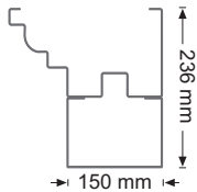
Trave perimetrale perimetral beam
