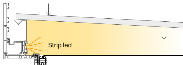
Pannelli coibentati di colore grigio chiaro Light grey insulated panels Panneaux isolants de couleur gris clair Illuminazione integrata (optional) Integrated lighting system (optional) Éclairage intégré (facultative)
