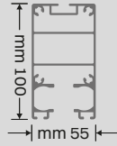
3 Guida Rail Rail
